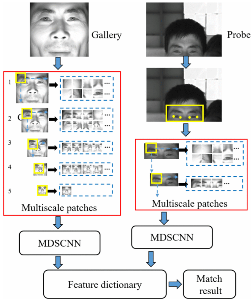
Figure 3.12: Multiscale double supervision convolutional neural network workflow with patch-to-patch matching to find the minimum matching object [90]
