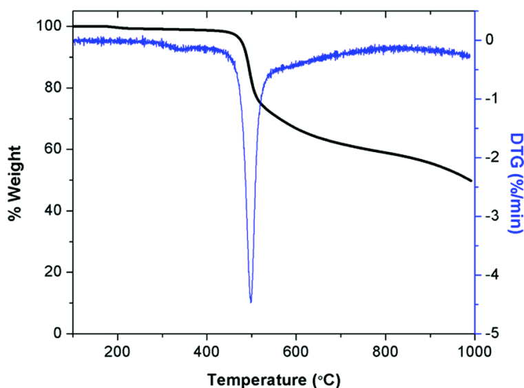
Figure 3.2. TGA and DTG curve [54]
