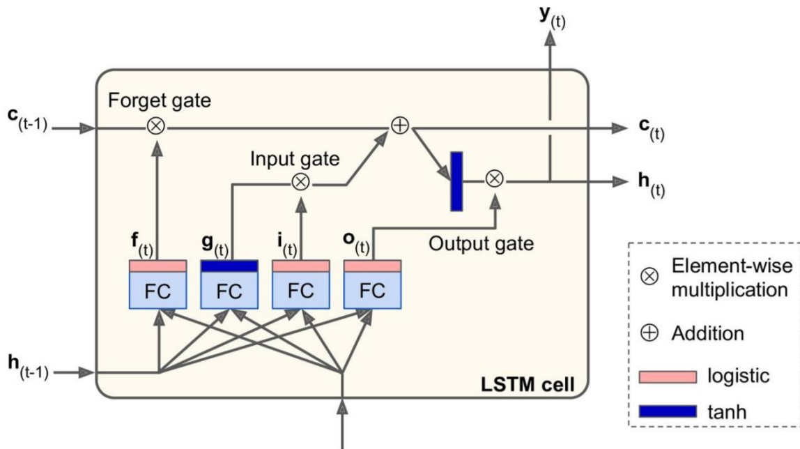
Figure 22: LSTM [20]
