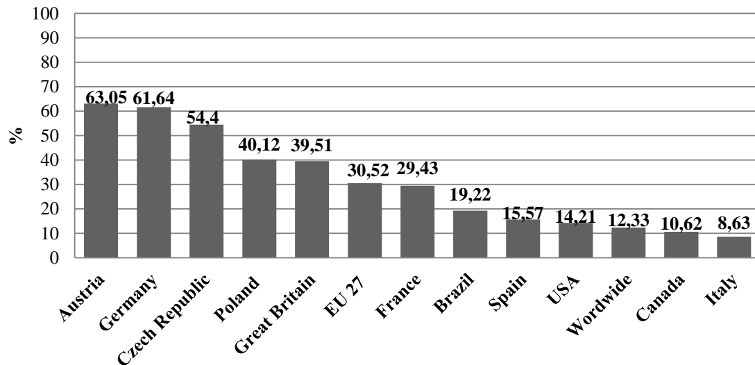
Chart 3: rate of fossil fuels replacement by SRF usage
