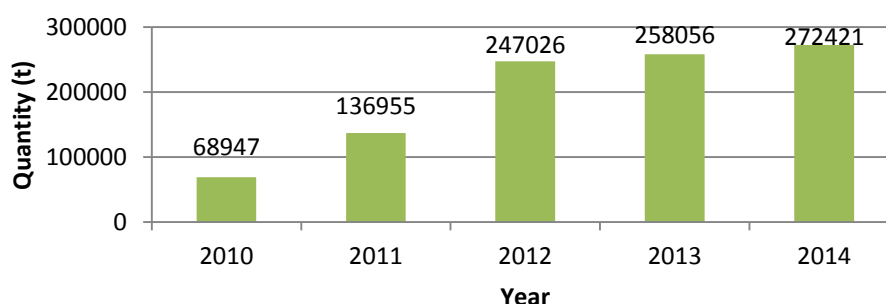
Chart 7: Quantities of municipal waste sent directly to the recovery in the period from 2010. to 2014.
