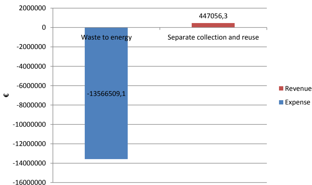
Chart 10: Graphic representation of the sum of all the expenses and revenues variants
