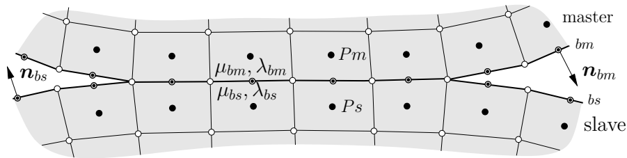
Figure 4.2. Conformal discretisation at contact interface
