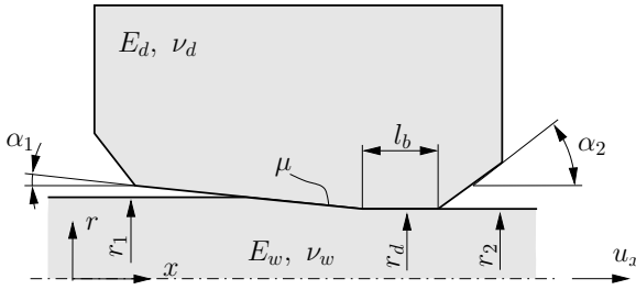
Figure 5.34. Wire drawing: problem geometry
