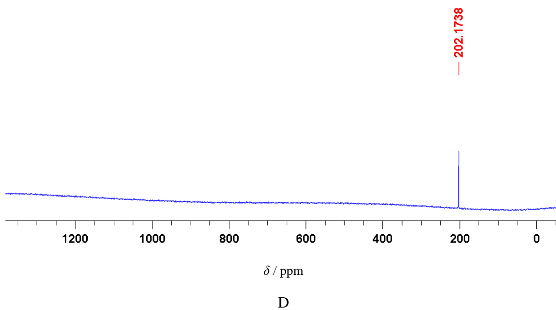
Slika D52. A) ^1\text{H} , B) ^{13}\text{C} , C) ^{15}\text{N} i D) ^{109}\text{Ag} spektri kompleksa [\text{Ag}(\text{NO}_3)(3\text{-Ipy})_2] , (K6).
