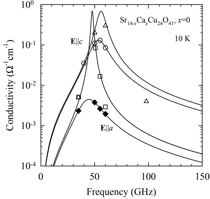
Figure 1.17 – Low-temperature microwave conductivity spectra at 10 K of single crystals taken from different batches of \text{Sr}_{14}\text{Cu}_{24}\text{O}_{41} , \mathbf{E} \parallel c and \mathbf{E} \parallel a . The full lines are based on fits to Lorentzians with characteristic frequencies of \Omega_c \approx 1.8 \text{ cm}^{-1} , \Omega_a \approx 1.7\text{--}3.5 \text{ cm}^{-1} . The modes are interpreted as evidence for CDW pinned mode in ladders. Data taken from Kitano et al. [15]
