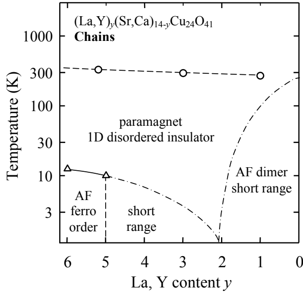
Figure 1.19 – Phase diagram of chains in the underdoped (\text{La}, \text{Y})_y(\text{Sr}, \text{Ca})_{14-y}\text{Cu}_{24}\text{O}_{41} materials. From Vuletić et al. [2]
