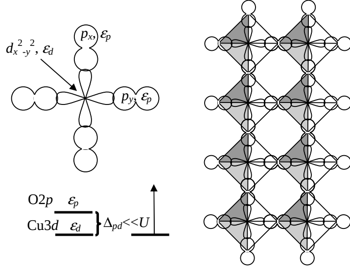
Figure 2.5 – Hybridization of the \text{O}2p^5 hole and \text{Cu}3d^9 hole within the \text{CuO}_4 square. At the oxygen sites only one of the two orbitals ( p_x or p_y ) is shown. The splitting of the energy levels is denoted on the lower left side. On the right, the squares assembled into a ladder structure are shown. From Vuletić et al. [2]
