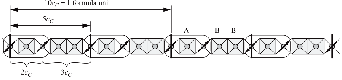
Figure 1.15 – Antiferromagnetic dimers (ovals) form in a cuprate chain with 6 holes and 4 spins per 10 Cu sites. This situation is similar to \text{Sr}_{14-x}\text{Ca}_x\text{Cu}_{24}\text{O}_{41} at small x where hole count on chains is close to 6. After Vuletić et al. [2]
