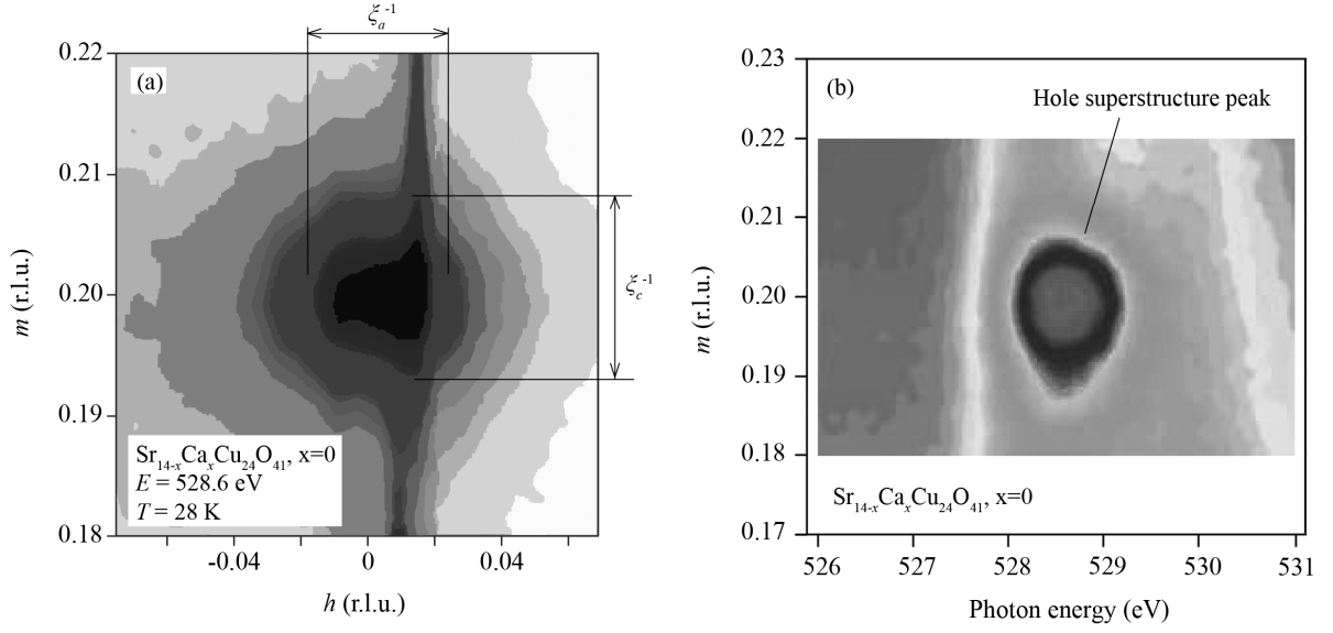
Figure 1.18 – (a) Reciprocal ladder space map around (h, k, m) = (0, 0, 0.2) with the X-ray energy tuned to the ladder hole absorption feature (MCP at 528.6 eV) taken at T = 28 K in \text{Sr}_{14-x}\text{Ca}_x\text{Cu}_{24}\text{O}_{41} , x=0 . Inverse coherence length \xi_c^{-1} and \xi_a^{-1} are denoted. (b) Hole super-structure peak intensity across the oxygen K edge. After Ref. [16].
