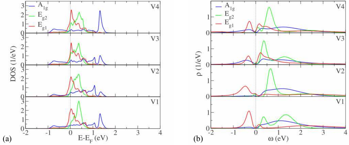
Figure 1.8 – t_{2g} manifold in the monoclinic insulating phase: (a) LDA DOS and (b) DMFT spectral functions (see text). From Lechermann et al. [45]
