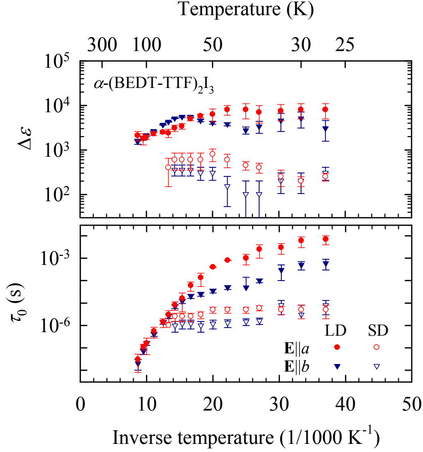
Figure 6.11 – Dielectric strength (upper panel) and mean relaxation time (lower panel) in \alpha -(BEDT-TTF) _2 I _3 as a function of inverse temperature; full and empty symbols represent parameters of the large and small dielectric mode, respectively, for \mathbf{E} along the a - (red circles) and b -axis (blue triangles).
