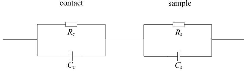
Figure A.1 – Two-contact measurements need to take into account the contribution of contacts (resistance R_c and capacitance C_c ) together with bulk properties of the sample (resistance R_s and capacitance C_s ).
