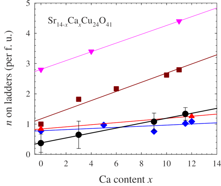
Figure 1.13 – The number of holes n per formula unit in the ladder subsystem vs. Ca content x in fully doped \text{Sr}_{14-x}\text{Ca}_x\text{Cu}_{24}\text{O}_{41} as determined by various experimental techniques: optical conductivity [72] (brown squares), NEXAFS [14] (blue diamonds), NMR [73] (red triangles), x-ray absorption [74] (pink triangles) and Hall effect measurements [75] (black circles). After Tafra et al. [75]
