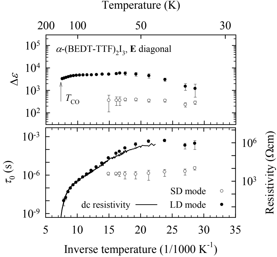
Figure 6.10 – Dielectric strength (upper panel) and mean relaxation time with dc resistivity (points and line, respectively, lower panel) in \alpha -(BEDT-TTF) _2 I _3 as a function of inverse temperature, for \mathbf{E} \parallel [1\bar{1}0] .
