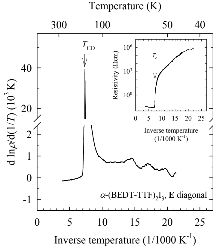
Figure 6.8 – Logarithmic resistivity derivative (main panel) and resistivity (inset) vs. inverse temperature of \alpha\text{-(BEDT-TTF)}_2\text{I}_3 for \mathbf{E} \parallel [1\bar{1}0] , i.e., in the diagonal direction of the ab plane.
