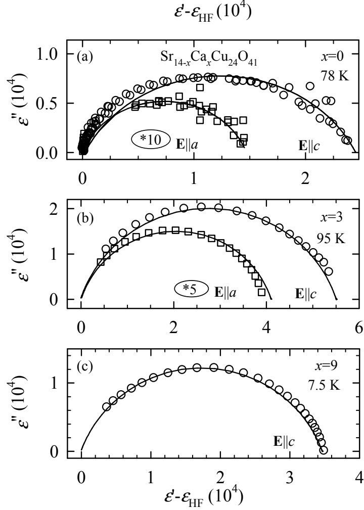
Figure 1.16 – Representative Cole–Cole plots of the real ( \epsilon' ) and imaginary ( \epsilon'' ) parts of the dielectric function of \text{Sr}_{14-x}\text{Ca}_x\text{Cu}_{24}\text{O}_{41} for x = 0 (a), x = 3 (b) and x = 9 (c) with the \mathbf{E} \parallel c and \mathbf{E} \parallel a . The plots for the response along the a -axis are scaled up by factors of 10 ( x = 0 ) and 5 ( x = 3 ). The full lines are fits of the generalized Debye function (refer to Eq. 3.2 in Sec. 3.2). The broad dielectric relaxation is associated with the overdamped longitudinal phason mode of ladder CDW. After Vuletić et al. [17]
