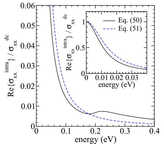
FIG. 11. (Color online) Solid line: the real part of the intraband conductivity (50) for E_F = 0.45 eV. The parameters are the same as in Fig. 10, with \delta M_{\alpha}^i(\omega) = \tilde{a} + |\hbar\omega|\tilde{b} and \tilde{a} = 0.01 eV, \tilde{b} = 0.015 . Dashed line: the result of the relaxation-time approximation, Eq. (51), for \hbar\Gamma_{\alpha} = 14 meV.
