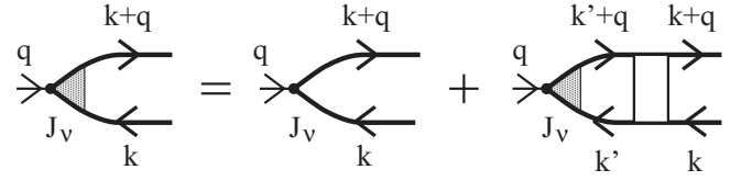
FIG. 4. The Bethe-Salpeter equation for the auxiliary electron-hole propagator \Phi_v^0(\mathbf{k}, \mathbf{k}_+, i\omega_n, i\omega_{n+}) . The white rectangle represents the irreducible four-point interaction U^0(\mathbf{k}_+, \mathbf{k}', \mathbf{k}'_+, \mathbf{k}, i\omega_m, i\omega_{m+}, i\omega_n) .
