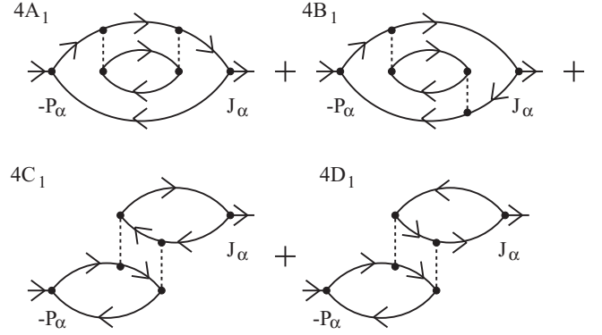
FIG. 7. The first set of four mutually related contributions to \sigma_{\alpha\alpha}^{(2)}(\omega) that are proportional to (H'_2)^2 [or (H'_1)^4 ].
