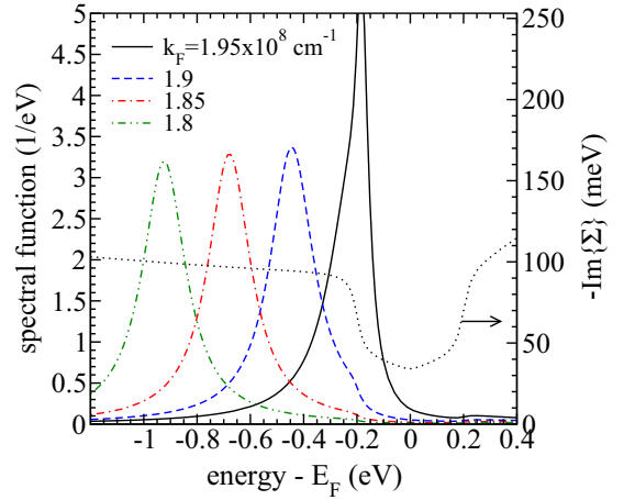
FIG. 3. (Color online) The spectral function (1/2\pi)\mathcal{A}(\mathbf{k}, \varepsilon) in the \pi^* band for \mathbf{k} = (k_x, 0) , k_x = 1.8, 1.85, 1.9 , and 1.95 \text{ \AA}^{-1} . Dotted line: the damping function -\hbar\Sigma^i(\mathbf{k}, \omega) . The parameters are the same as in Fig. 2, with \hbar\delta\Sigma^i(\mathbf{k}, \omega) = a + |\hbar\omega|b , and a = 0.03 \text{ eV} , b = 0.05 .
