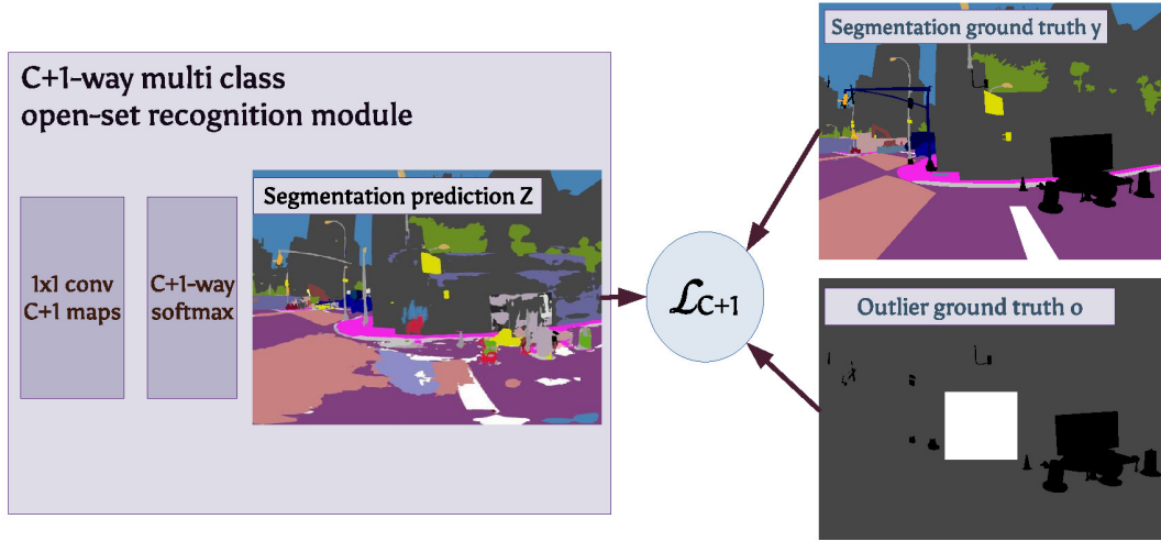
Figure 4.5: C+1-way multi-class recognition module is trained as a standard segmentation module, where negative examples get classified as the C+1-st class.
