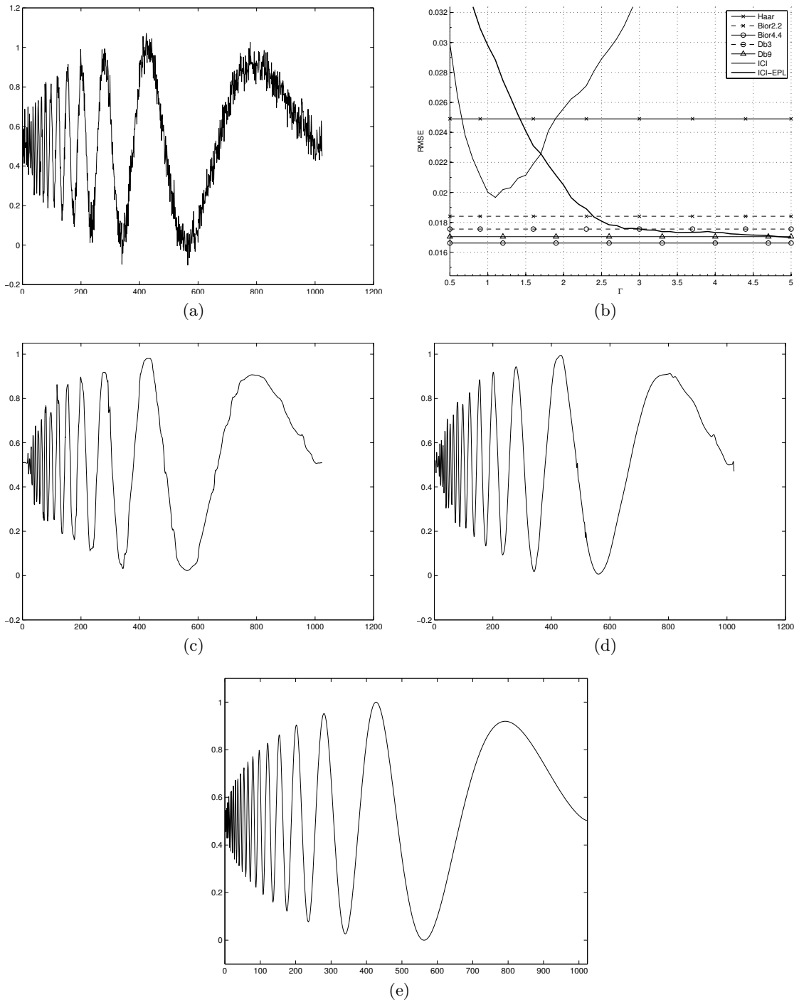
Figure 3.20: Doppler signal corrupted by noise with \sigma_\epsilon = 5\% of total signal magnitude (a), average RMSE for various denoising methods (b) signal denoised by optimal wavelet transform ( Bior4.4 ) (c), signal denoised by the ICI-EPL (d) and original signal (e)
