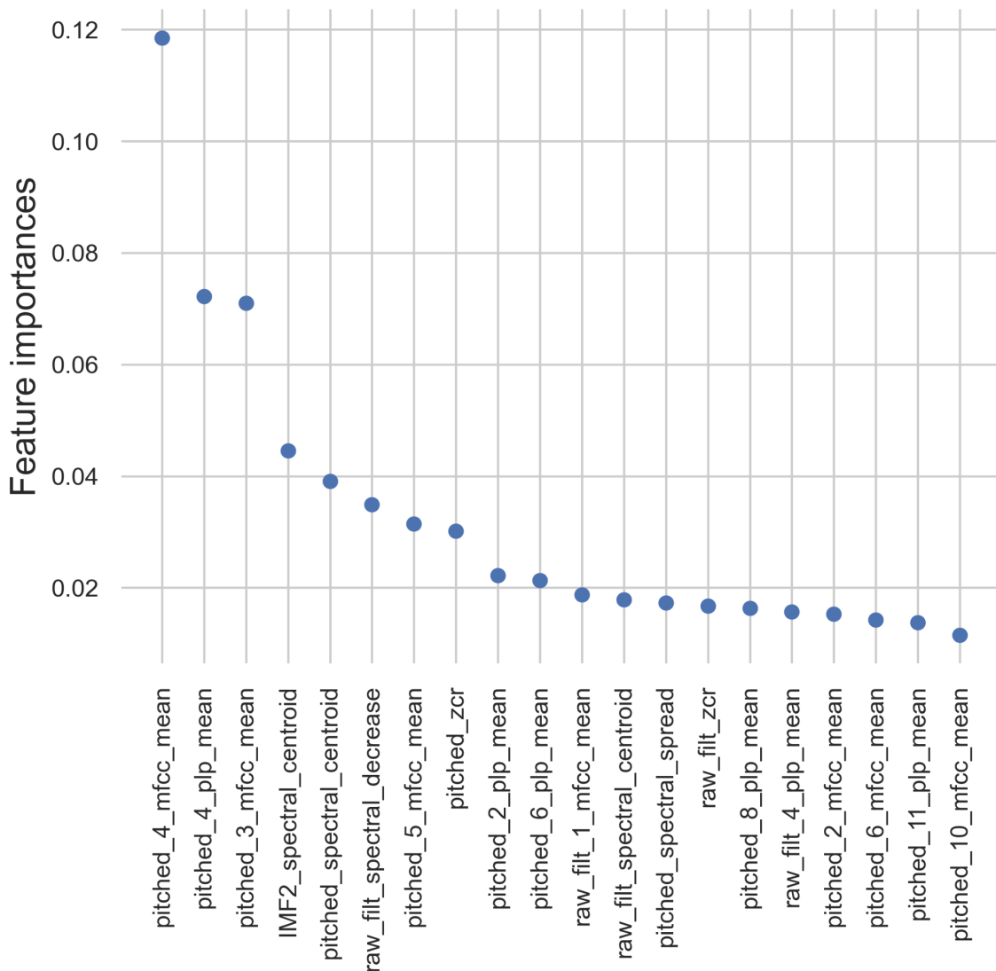
Figure 4.17. The top 20 features inherently obtained by the learning algorithm of the random forest classifier. Simulated dataset with -22 dB SNR used as an input.
