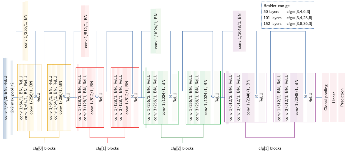
Figure 2.5: We illustrate the ResNet architecture which consists of residual blocks. Each block comprises several convolution and normalization layers. The layer input and output are connected through skip connection and merged with addition. The full network is created through the stacking of residual blocks. The blocks are organized into groups, with spatial resolution halving between two successive groups.
