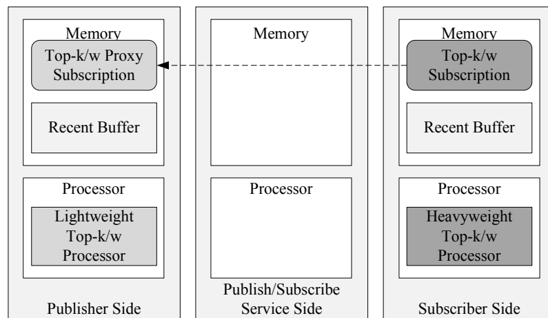
Figure 5.6: Centralized top-k/w publish/subscribe system with subscription flooding.
