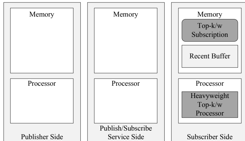
Figure 5.5: Centralized top-k/w publish/subscribe system with publication flooding.
