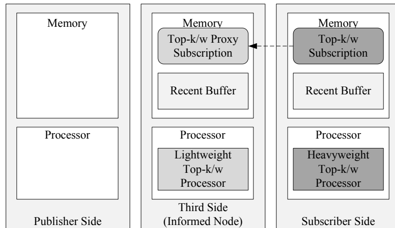
Figure 6.15: Distributed top-k/w publish/subscribe system with informed gossiping.
