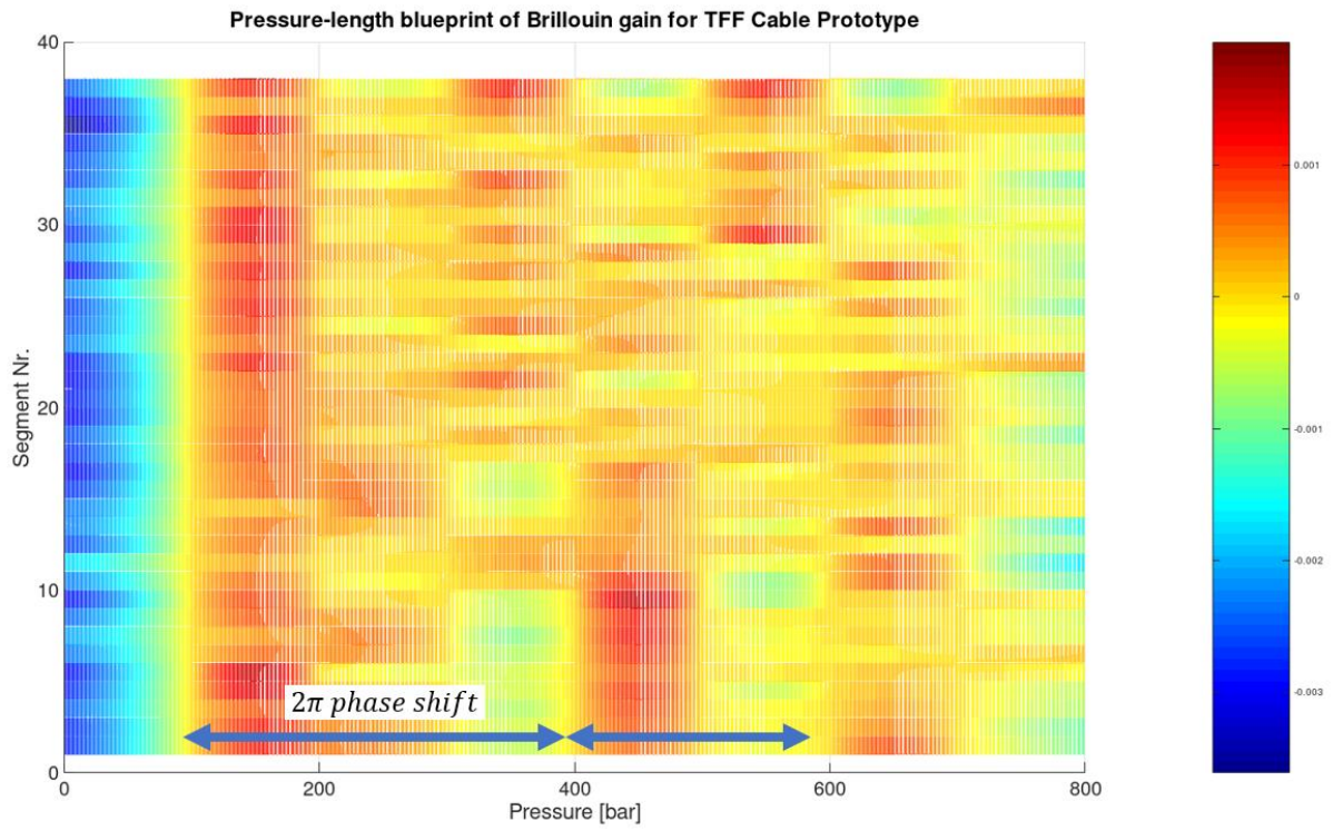
Figure-4.17: Mesh representation of Brillouin gain derivative in \Delta k_z -plane revealing 2\pi phase periods. The minimums are found in the transition zones from yellow to red, in the direction left to right. The distance from two adjacent minimums corresponds to 2\pi phase shift.
