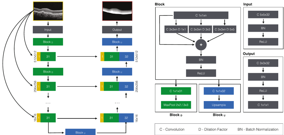
Fig. 3.4 BRU-net (Branch Residual U-Net). [74]
