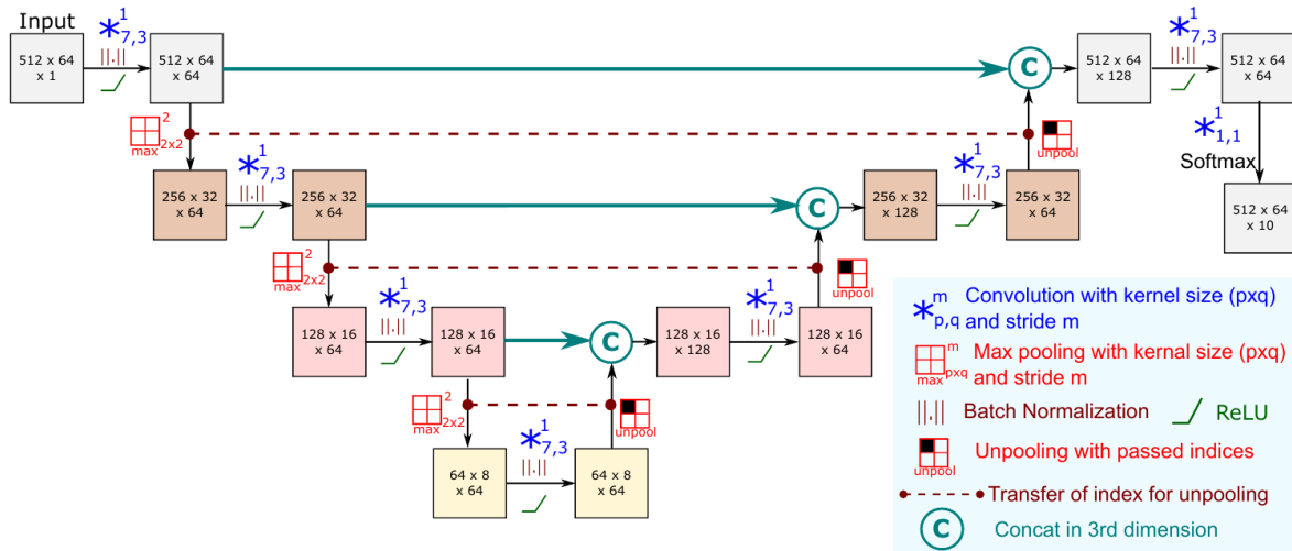
Fig. 3.8 ReLayNet architecture. [46]
