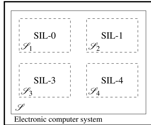
(b) Functions of different criticality level are scheduled with local schedulers \mathcal{S}_1, \mathcal{S}_2, \mathcal{S}_3, and \mathcal{S}_4 on dedicated processors based on criticality. Scheduler \mathcal{S} determines the global schedule.
