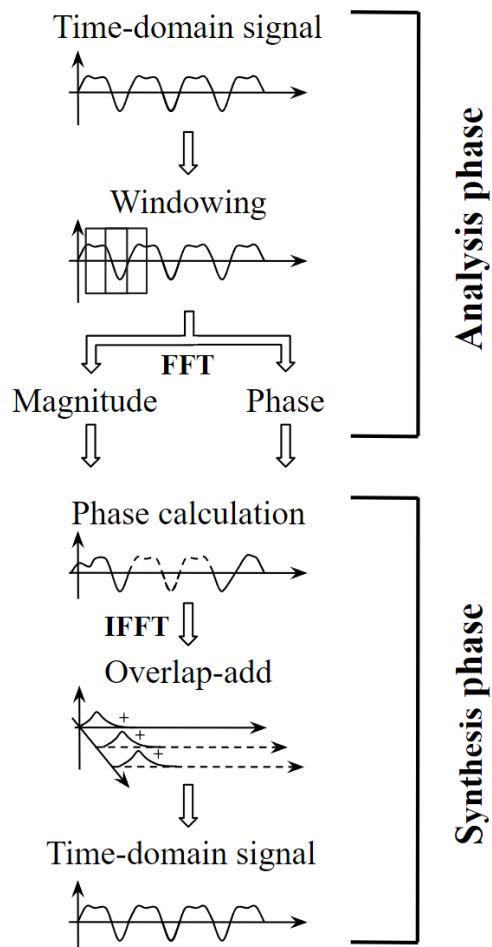
Figure 2.4. Pitch shifting algorithm flowchart
