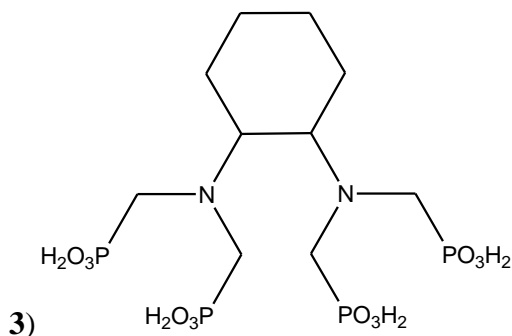
Figure 12. Compound 3.
