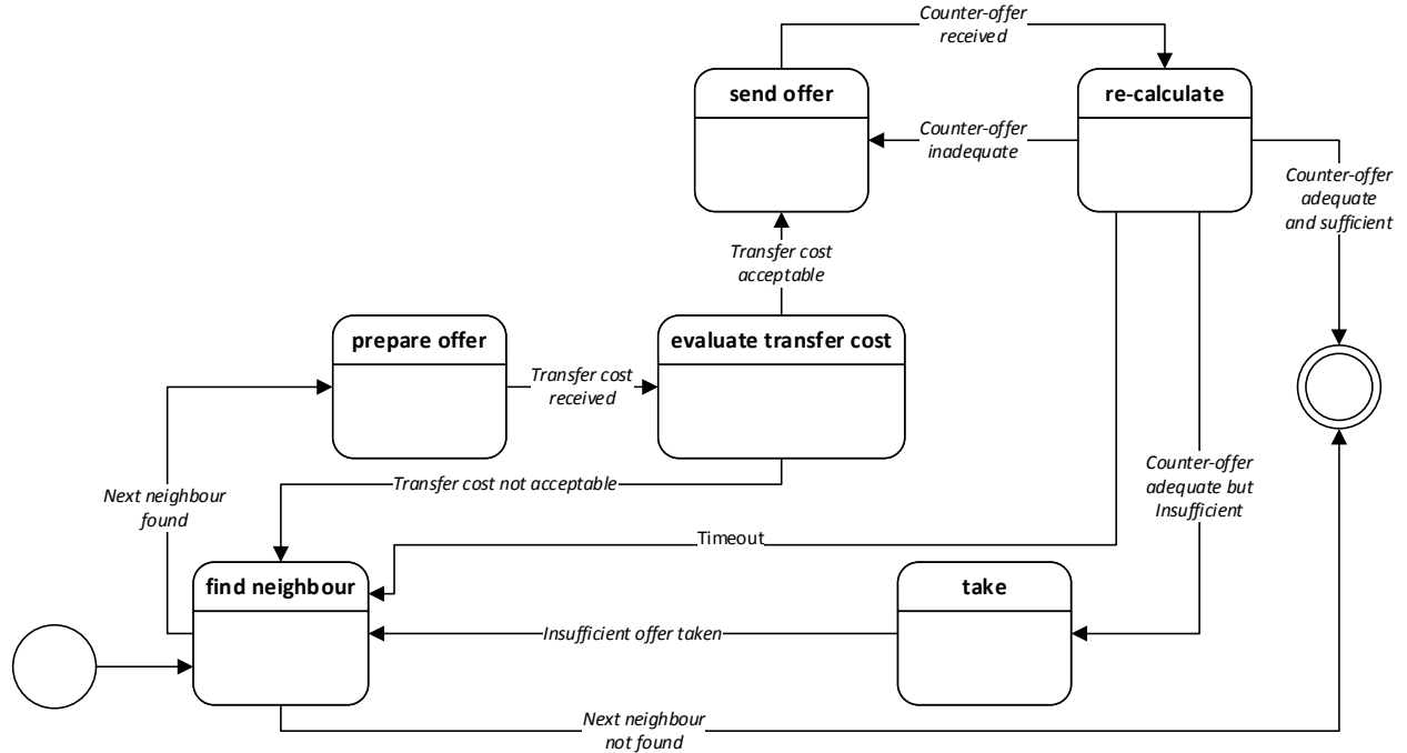
Figure 10. A finite state machine of the negotiating client
