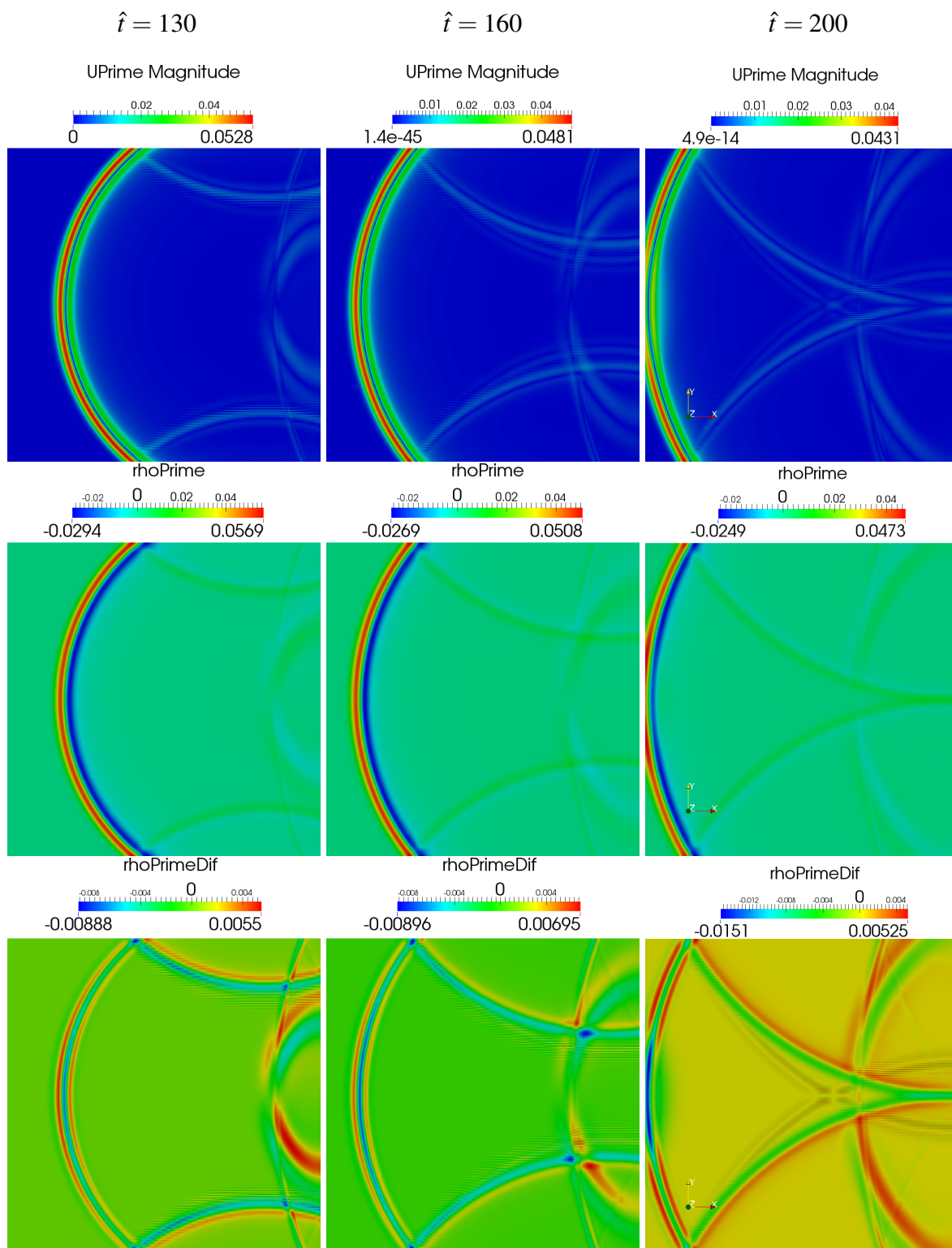
Figure 6.1.4: Acoustic fields: velocity fluctuation magnitude, |\hat{\mathbf{U}}'| (top), density fluctuation, \hat{\rho}' (middle), difference between \hat{\rho}'_{\text{analytical}} and \hat{\rho}'_{\text{numerical}} (bottom), 1 000 000 cell grid.
