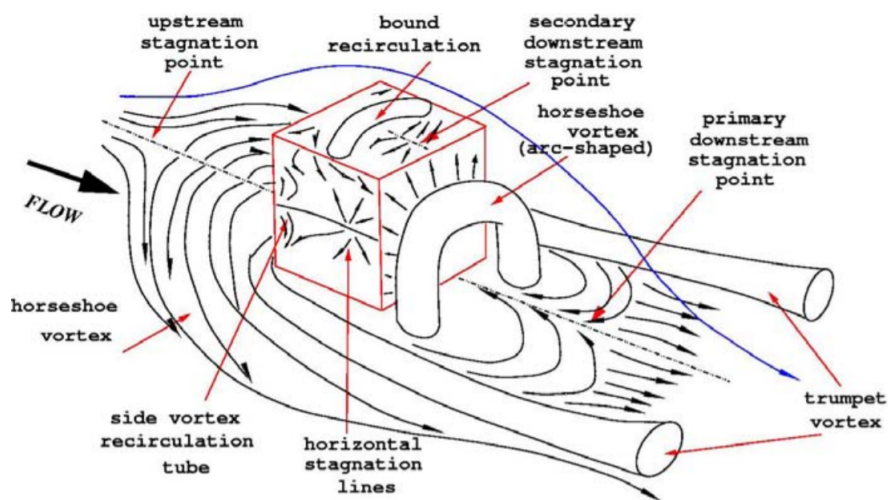
Figure 2.15: 3D representation of the flow around a surface mounted cube, [31]
