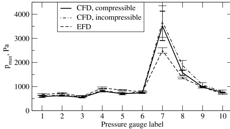
Figure 2.8: Comparison of average pressure peaks for the green sea loading case (PAPER 6).
