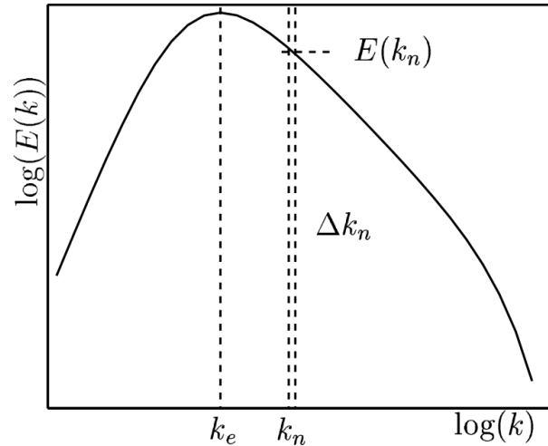
Figure 3.4.1: Model spectrum [15].
