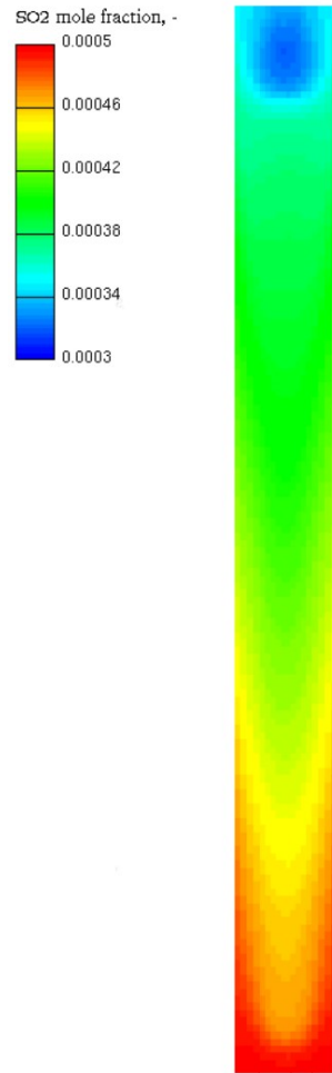
Figure 3.23: SO 2 concentration on the cross-section. Gas flow 40m 3 /h; pure water flow 0.1 m 3 /h.
