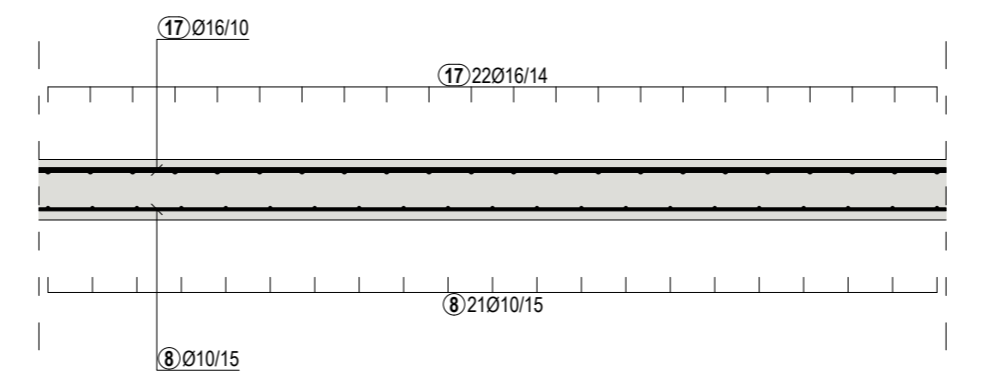
2-2 R=1:25
