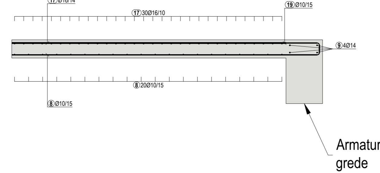
1-1 R=1:25
