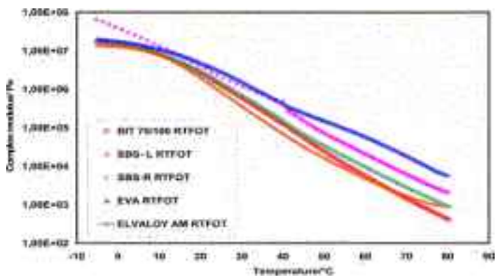
Figure 4 Complex modulus as a function of temperature for BIT 70/100 and PmBs after RTFO
