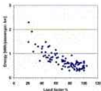
Figure 8 Aircraft: energy used with passenger load factor
