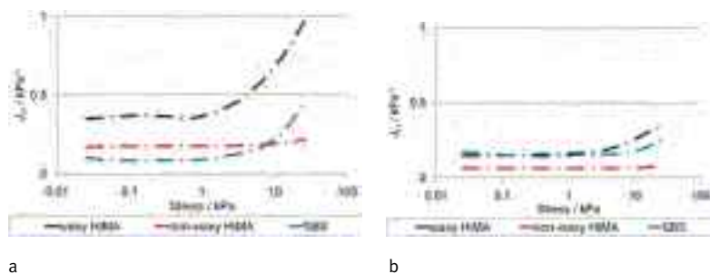
Figure 6 (a) Non-recoverable compliance at different stress levels of bituminous binders at 55°C. (b) Non-recoverable compliance at different stress levels of bituminous binders after RTFO-aging at 55°C.
