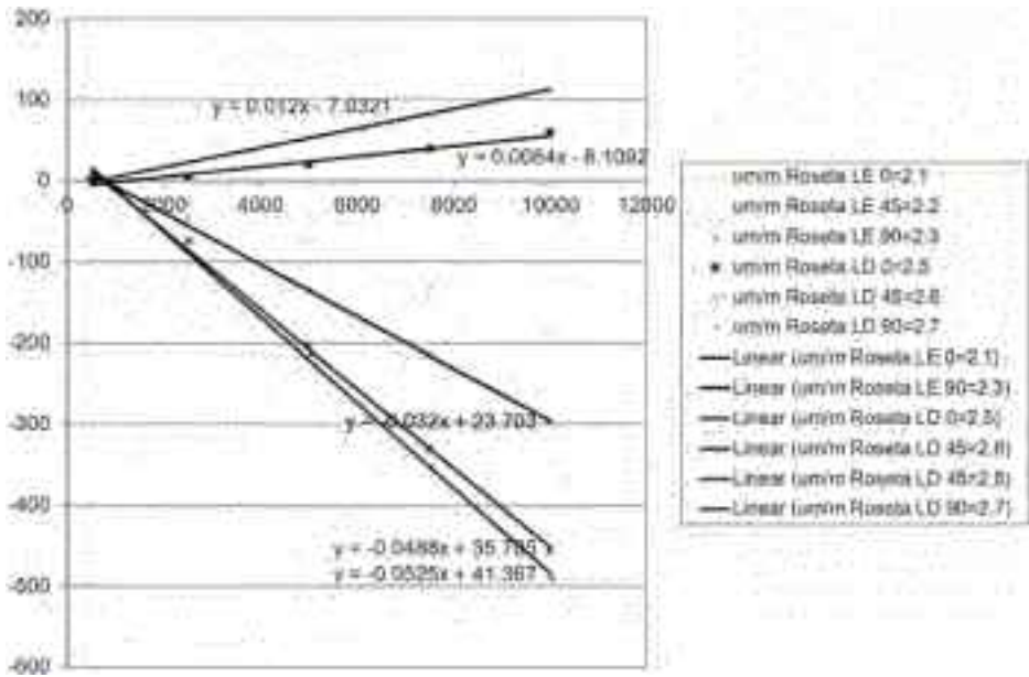
Figure 5 Equation for rosette calibration: \mu\text{s} to kg
