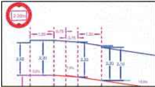
Figure 6 Example for calculating headroom along a garage ramp (5 cm construction tolerance not included!)
