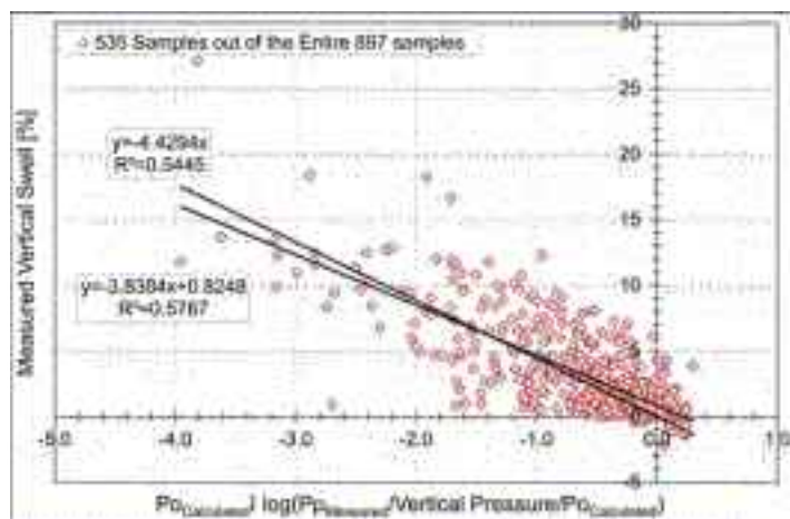
Figure 3 Measured vertical swelling versus Po \times \log(Pp/Po) of 535 undisturbed samples, where Po is the calculated swelling–pressure according to eqn (5) and Pp is the measured (applied) vertical pressure
