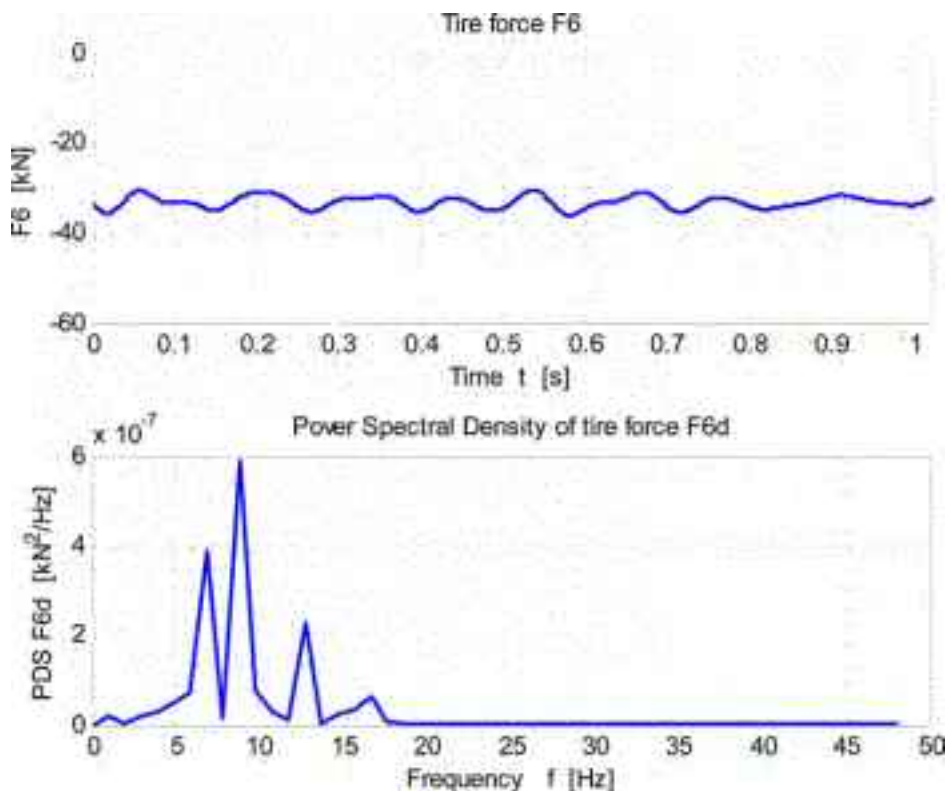
Figure 10 Tire force F_6(t) and its PSD, \Phi_0 = 4 \cdot 10^{-6} \text{ m}^2/(\text{rad}/\text{m})
