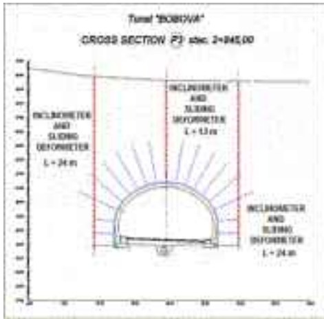
Figure 4 Measuring profile of the Bobova Tunnel with designated positions of the installed inclinometers and deformaters
