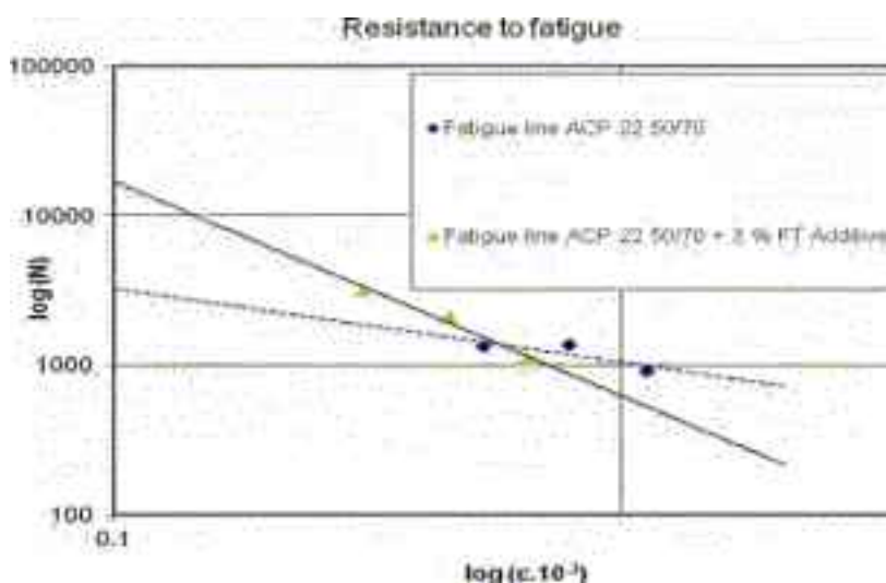
Figure 3 Resistance to fatigue of the asphalt mixtures
