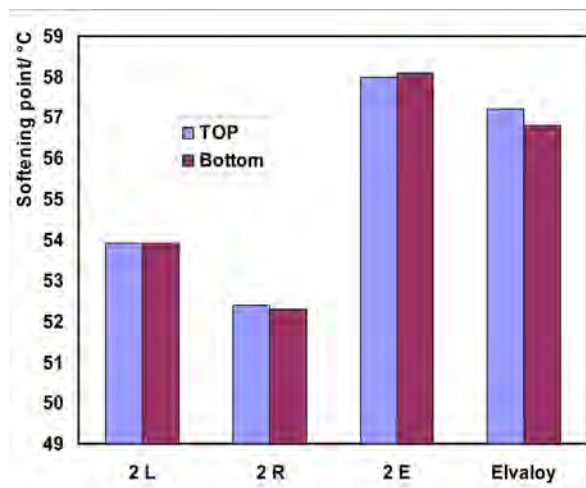
Figure 8 Storage stability
