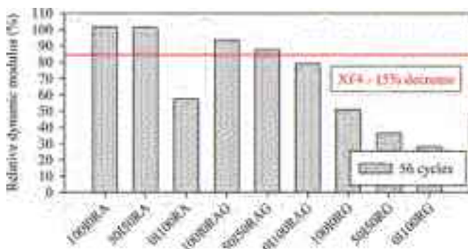
Figure 6 Resistance of concrete to freeze-thaw cycles without salt
