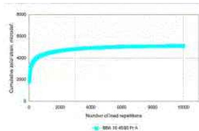
Figure 3 BBA 16 asphalt mixture creep curve
