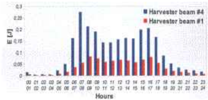
Figure 8 Power distribution for Friday, 4 November 2011
