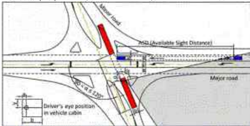
Figure 2 The scheme of the intersection for the calculation of available sight distance (ASD)
