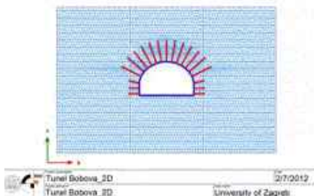
Figure 2 Numerical model of the Bobova Tunnel used in 2D analysis
