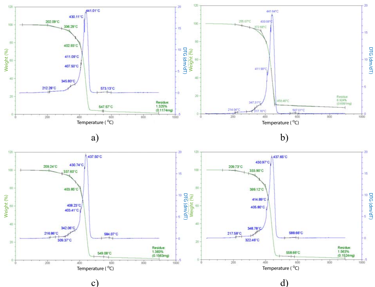
Figure 41. TG and DTG curves for Cosmolight QS photopolymer samples:
