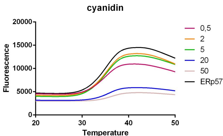
Figure 32. Changes in SYPRO orange fluorescence with the increase in temperature observed for the protein alone and in presence of different flavonoid concentrations (0.5, 2, 5, 20, 50 \mu M)
