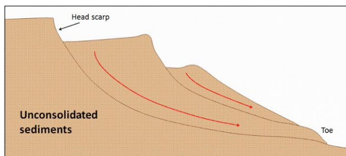
Slika 1. Prikaz kretanja nekonsolidiranih sedimenta to jest slampiranja (internetski izvor: https://opentextbc.ca/geology/chapter/15-2-classification-of-mass-wasting/ ; 15.05.2021.).
