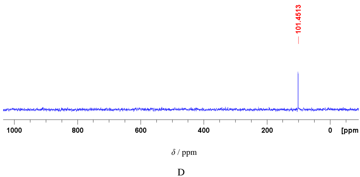
Slika D32. A) ^1\text{H} , B) ^{13}\text{C} , C) ^{15}\text{N} i D) ^{109}\text{Ag} spektri spoja [\text{Ag}(\text{NO}_3)(2\text{-Clpy})_2] , (K1).
