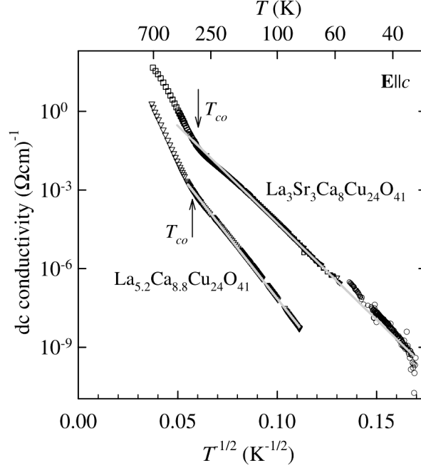
Figure 1.20 – The dc conductivity along the c -axis in the underdoped (\text{La}, \text{Y})_y - (\text{Sr}, \text{Ca})_{14-y} \text{Cu}_{24} \text{O}_{41} , y = 3, 5 . The low-temperature conductivity is in the one-dimensional variable-range hopping regime characterized by the temperature dependence \sigma_{\text{dc}} \propto \exp -(T_0/T)^{1/(1+d)} , d = 1 . From Vuletić et al. [2]
