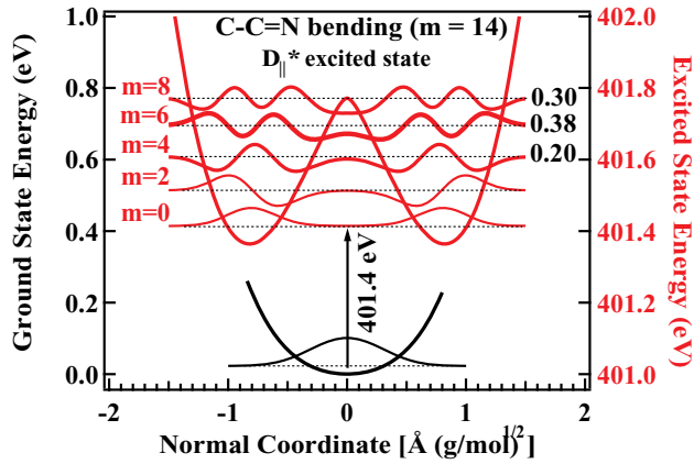
FIG. 4. (Color online) Ground state (black solid line), D_{\parallel}^* excited state (orange) potential surface of its most excited, C-C \equiv N out-of-plane bending vibrational mode ( m = 14 ). Corresponding wave functions (solid lines) and eigenvalues (dashed lines) are drawn for each potential. The arrow indicates a vertical transition (at q = 0 ) between \psi_0 and \psi'_0 . The probability of the excitation of the three most important quantum states is indicated at the right side of the excited potential.
