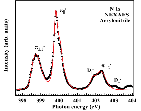
FIG. 2. (Color online) The entire experimental N 1s NEXAFS spectrum (black points) of the acrylonitrile molecule compared to calculations including vibrational analysis (red line). The spectra show two strong low-energy structures ( \pi_{\perp 1}^* and \pi_{\parallel}^* ), a D_{\parallel}^*-\pi_{\perp 2}^* doublet and a small D_{\perp}^* structure close to the ionization potential. Experimental details are given in Ref. [17].
