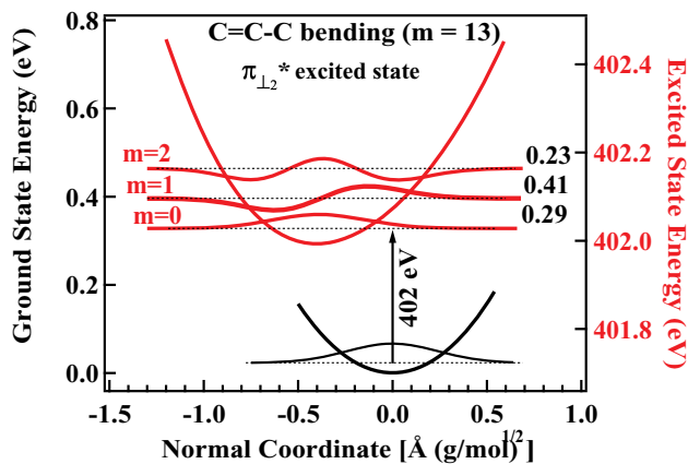
FIG. 5. (Color online) Ground state (black), \pi_{\perp}^* excited state (orange) potential surface projected to its second most excited, out-of-plane C=C-C bending vibrational mode ( m = 13 ). Wave functions and eigenvalues are indicated. The probability of the excitation to the three states with most important Franck-Condon factors is indicated at the right side of the excited potential.
