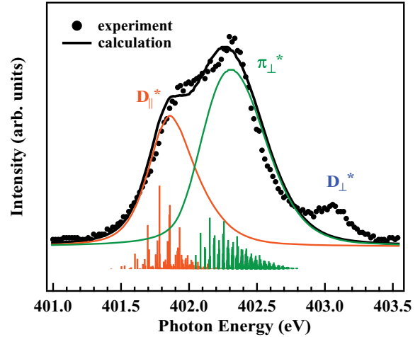
FIG. 6. (Color online) Calculation of the 401.5- to 402.5-eV doublet compared to the experiment. It is composed of vibrational progressions of the D_{\parallel}^* excited state (orange line, maximum at 401.9 eV) and the \pi_{\perp}^* excited state (green line, centered at 402.35 eV). Addition of these two structures (black line) matches experimental spectra well.
