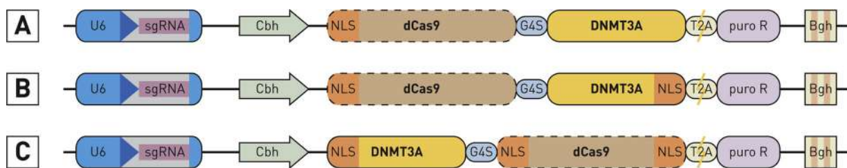
Fig. 1. Schematic representation of tested constructs. Different dCas9 orthologs were tested for DNMT3A activity at the targeted sites. The basic configuration included DNMT3A fused to dCas9 orthologs at their Ctermini, either without (A) or with (B) an additional nucleoplasmin NLS at the C-terminus of the DNMT3A catalytic domain. Additionally, fusion of DNMT3A at the N-terminus of dSpCas9 and dSaCas9 was tested (C).
