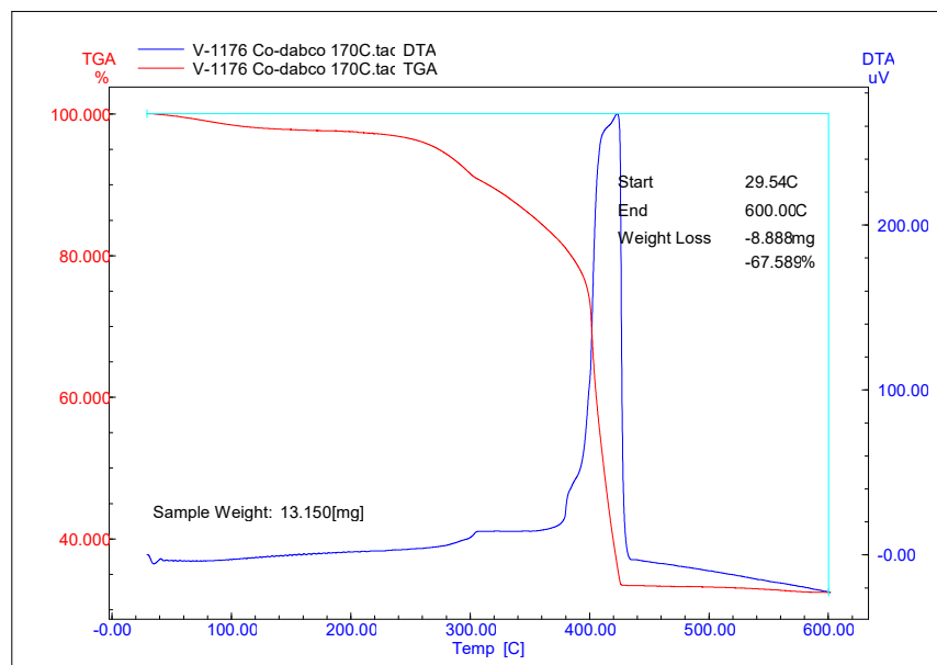
Slika 49. DTA i TGA krivulje spoja \text{Co}_2(\text{BDC})_2(\text{DABCO})
