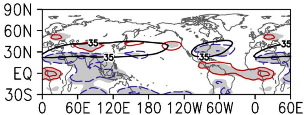
Appendix Figure A5 Changes of background states in the zonal wind on 200 hPa level ( u_{200} ) shown in colour contours (red - positive values, blue - negative values; contour interval = 1 m/s) in Jan/Feb from three selected control experiments (i.e., without El Niño anomaly forcing) of ICTP AGCM. 'Early' SST climatology and 'high' sea-ice concentration refer to the 1979-1999 period, while the 'late' SST climatology and 'low' sea-ice concentration refer to the 2005-2015 period. The 35 m/s isoline for mean u_{200} is indicated by the black line, roughly illustrating the cores of jet streams. Grey shading is applied at the 95% two-tail significance level.
