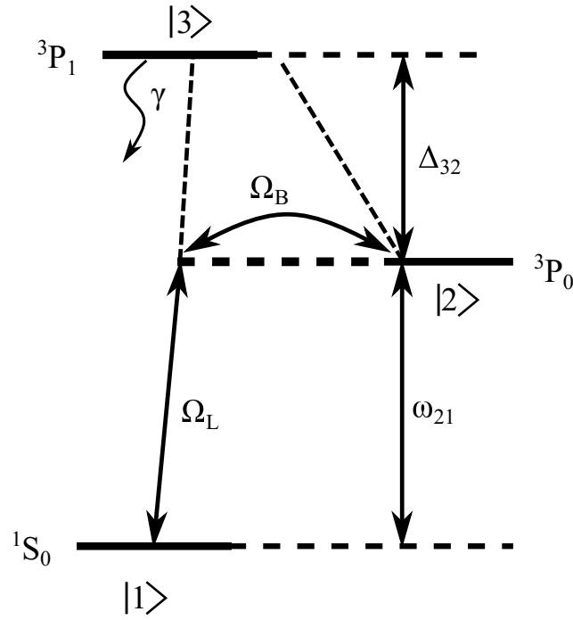
Figure 2.9: Magnetically induced spectroscopy of the forbidden clock transition in bosonic optical clock. The use of a strong bias magnetic field induces a coupling between the 3P_0 and 3P_1 state. Because of it, the upper clock state is no longer a pure state but a mixture of the two states. Due to this mixing, the bosonic clock transition becomes weakly allowed, enabling the operation of a bosonic optical clock. \Omega_B is the coupling matrix element between the two excited states due to the strong magnetic field, while \Omega_L is the matrix coupling element induced by the electric field of the clock transition probe beam. The clock transition is given by \omega_{21} , the detuning between the upper two states of the triplet is given by \Delta_{32} and decay rate from the 3P_1 state is given by \gamma . More details on magnetically induced spectroscopy are given in the main text and are available in Taichenachev et al. [83].
