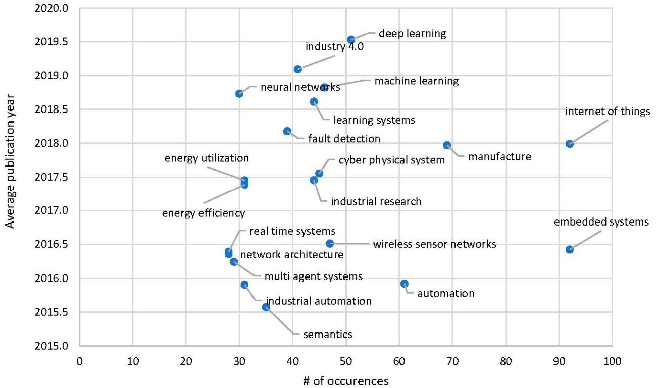
Figure 5. The occurrence and average publication year of the most frequent terms. Note: industrial informatics was not excluded.
