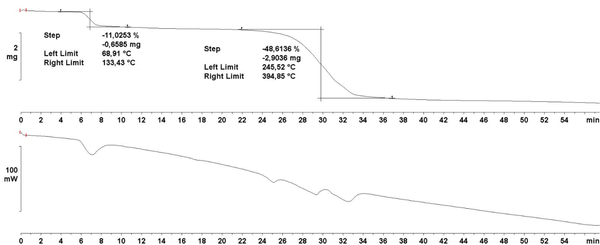
Slika D28. TG i DSC krivulje rac\text{-(DAP)}_2[\text{Mn}_2\text{Cl}_6(\text{H}_2\text{O})_4]\text{Cl}_2
