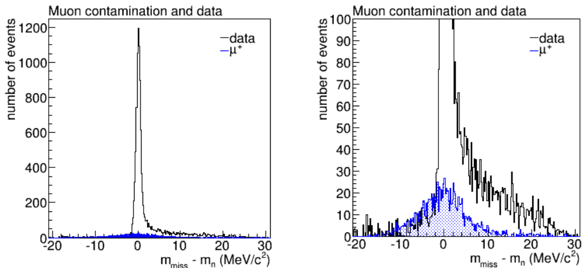
Figure 6.25 — The missing mass distributions of the background subtracted data (black) and of the muons from the pion decay simulation (blue) for the axialFF_591 setting. The total simulated distribution (pion + muon) was normalized with respect to the highest bin of the experimental distribution. The left and the right figure show same distributions, they only differ in ranges which are shown.
