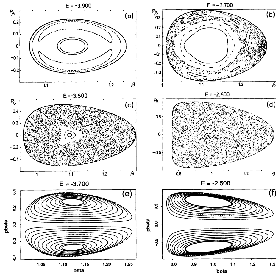
FIG. 1. (\beta, P_\beta) Poincaré surfaces of section for (a) \xi = 8, E/\kappa_2 = -3.90 , (b) \xi = 8, E/\kappa_2 = -3.70 , (c) \xi = 8, E/\kappa_2 = -3.50 , (d) \xi = 8, E/\kappa_2 = -2.50 , (e) \xi = 2, E/\kappa_2 = -3.70 , and (f) \xi = 2, E/\kappa_2 = -2.50 . Panels (e) and (f) correspond to the SU(3) dynamical symmetry and panels (a)–(d) to broken dynamical symmetry.
