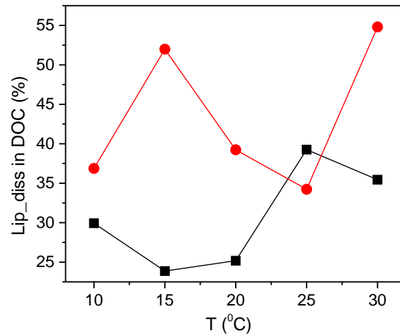
Fig. S1. Average contribution of dissolved lipids to DOC for the P-depleted (circles) and P-replete (squares) C. pseudocurvisetus growth conditions.
